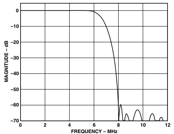
TPC 5. Extended Mode (SSAF) Luma Filter
