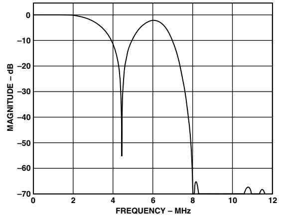
TPC 4. PAL Notch Luma Filter
