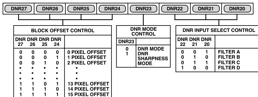
Figure 74. DNR Register 2
