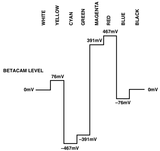
Figure 121. NTSC 100% Color Bars with Pedestal V
