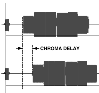
Figure 11. Chroma Delay
