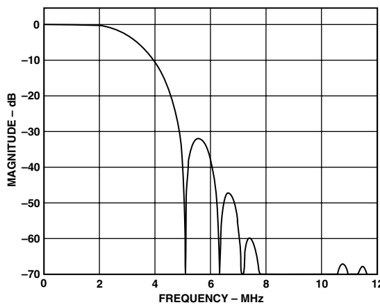
TPC 9. Luma CIF Filter
