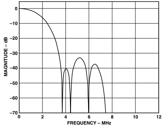
TPC 10. Luma QCIF Filter
