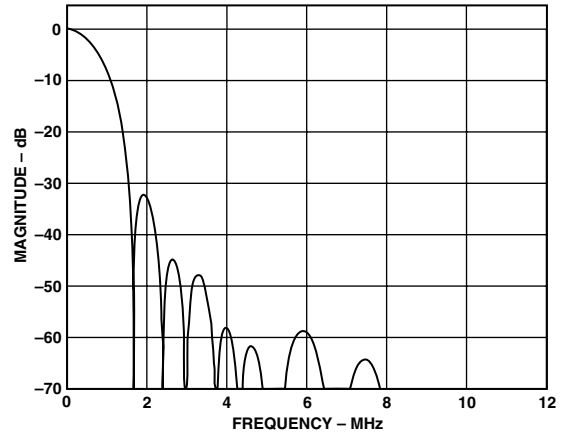
TPC 16. Chroma CIF Filter
