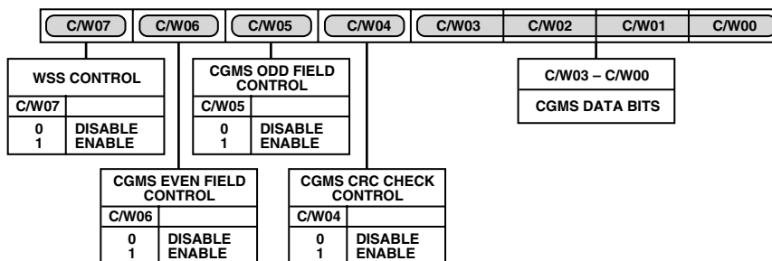
Figure 59. CGMS_WSS Register 0
