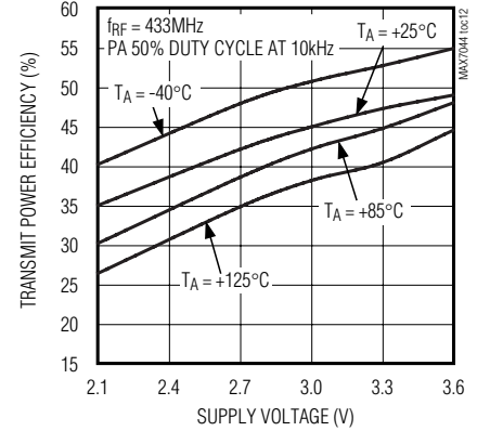
TRANSMIT POWER EFFICIENCY vs. SUPPLY VOLTAGE
