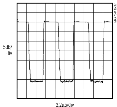
AM DEMODULATION OF PA OUTPUT DATA RATE = 100kHz
